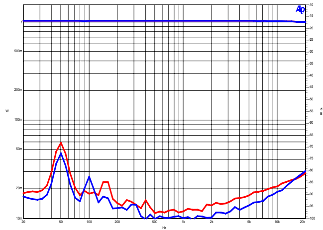
Crosstalk L/R // R/L 1 kHz / \geq 75 dB (-88,5 dB / -88,7 dB)
