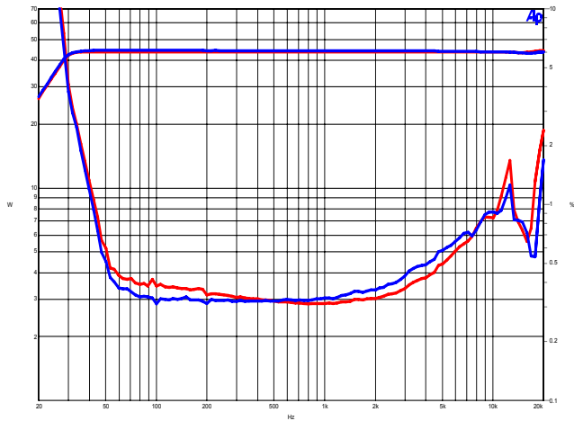
Distortion THD+N 2x 45 Watts / Sine 1kHz / typ. \leq 1\% (0,313% / 0,334%)
