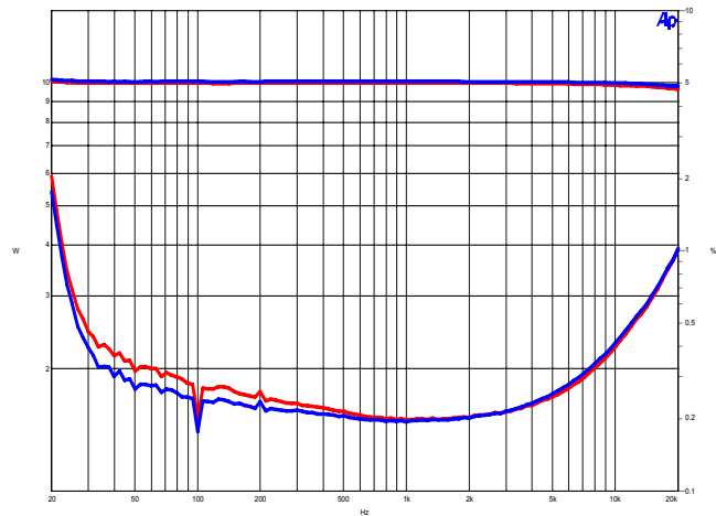
Distortion THD+N 2x 10 Watts / Sine 1kHz / typ. \leq 0,25\% (0,198% / 0,194%)
