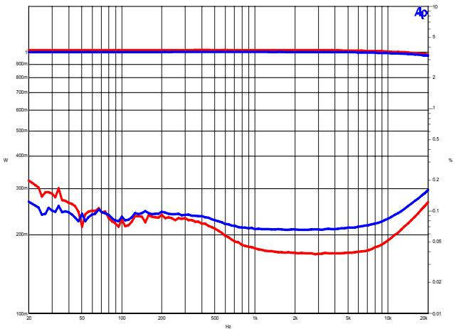
Distortion THD+N 2x 1 Watt / Sine 1kHz / typ. \leq 0,1\% (0,043%, 0,046%)
